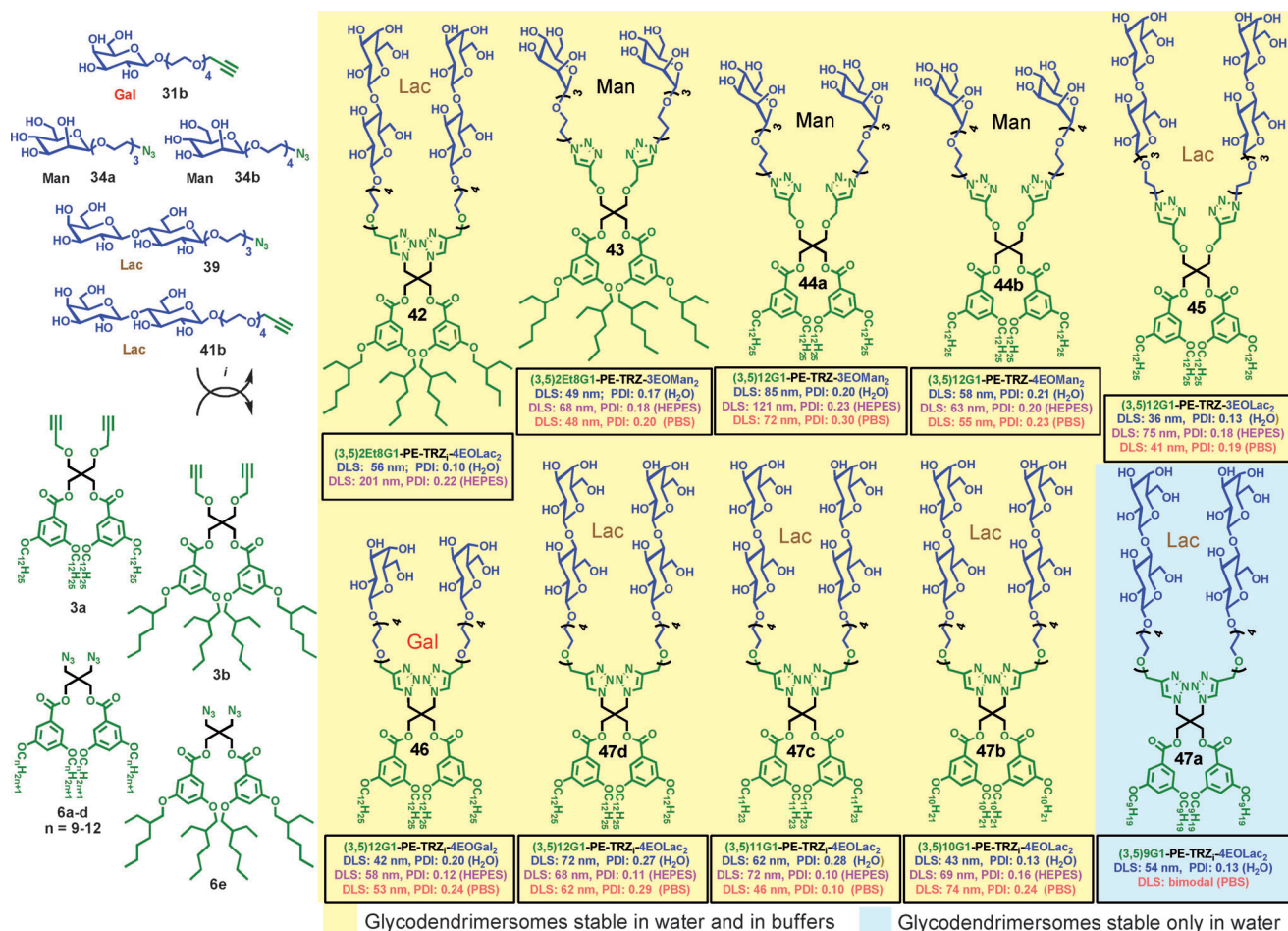
Scheme 1. Modular synthesis of library 1, which consists of ten constitutional isomeric twin-twin carbohydrate compounds with D-Man, D-Gal, and D-Lac as headgroups. Reagents and conditions: CuSO 4 ·5 H 2 O, sodium ascorbate, THF/water, 23 °C. The diameter (in nm) and polydispersity (PDI) of the glycodendrimersomes were measured by DLS in water and in HEPES and PBS (0.5 mg mL -1 ). THF = tetrahydrofuran, HEPES = 2-[4-(2-hydroxyethyl)-1-piperazinyl]ethanesulfonic acid, PBS = phosphate buffered saline.
