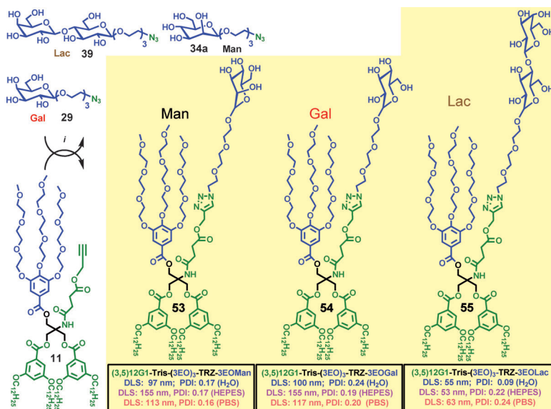
Scheme 3. Modular synthesis of library 3, which consists of three twin-mixed TEG:carbohydrate compounds with D-Man, D-Gal, and D-Lac as headgroups. Reagents and conditions: \text{CuSO}_4 \cdot 5\text{H}_2\text{O} , sodium ascorbate, THF/water, 23 °C. The diameter (in nm) and polydispersity (PDI) of the glycodendrimer vesicles were measured by DLS in water and in HEPES and PBS ( 0.5\text{ mg mL}^{-1} ).
