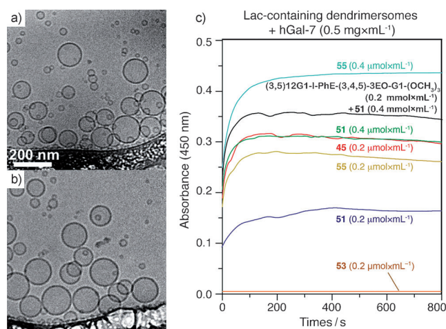
Figure 2. Representative cryo-TEM images of glycodendrimerosomes self-assembled by injection of THF solutions of a) 45 ( 0.5 \text{ mg mL}^{-1} ) in PBS or b) 50a ( 0.5 \text{ mg mL}^{-1} ) in HEPES. c) Agglutination assay with Lac-containing glycodendrimerosomes (in \mu\text{mol mL}^{-1} ) with different topologies in the presence of hGal-7 ( 0.5 \text{ mg mL}^{-1} ) in PBS buffer.
