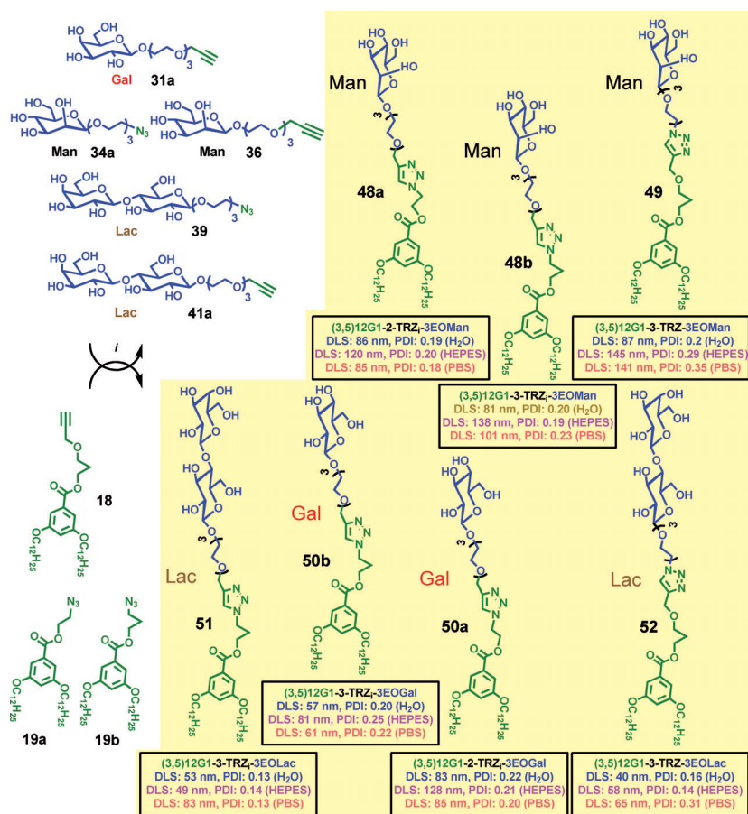
Scheme 2. Modular synthesis of library 2, which consists of seven constitutional single-single carbohydrate compounds with D-Man, D-Gal, and D-Lac as headgroups. Reagents and conditions: \text{CuSO}_4 \cdot 5\text{H}_2\text{O} , sodium ascorbate, THF/water, 23 °C. The diameter (in nm) and polydispersity (PDI) of the glycodendrimer vesicles were measured by DLS in water and in HEPES and PBS ( 0.5\text{ mg mL}^{-1} ).
